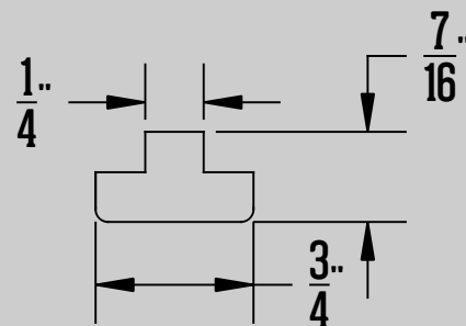
Mullion
